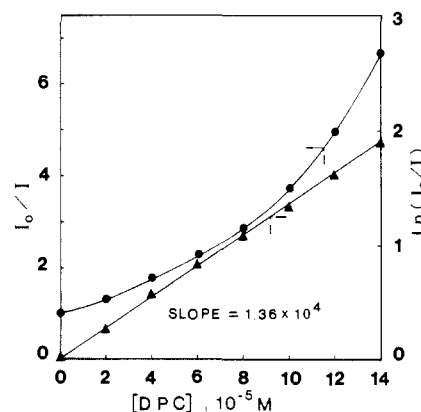
Figure 6. Quenching of pyrene fluorescence by DPC in PMA-deaerated aqueous solutions containing 8 \times 10^{-3} \text{ M} C_{10} TAB at pH 8, calculated from steady-state data. [PMA] = 1 g/L, [pyrene] = 2 \times 10^{-6} \text{ M} . I_0 and I are relative intensities of pyrene fluorescence in the absence of and in the presence of DPC, respectively. Note: Plot of I_0/I (●) vs. [DPC] is not linear, but plot of \ln(I_0/I) (▲) vs. [DPC] is linear and slope = 1.36 \times 10^4 .
