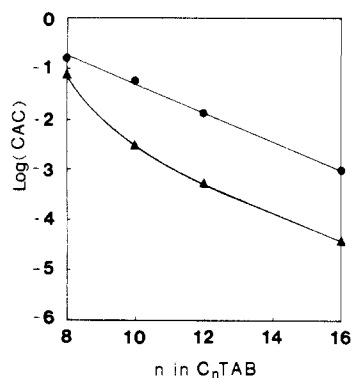
Figure 4. Plot of log(CAC) vs. n in C_n TAB (▲) and plot of log(cmc) vs. n in C_n TAB (●).
