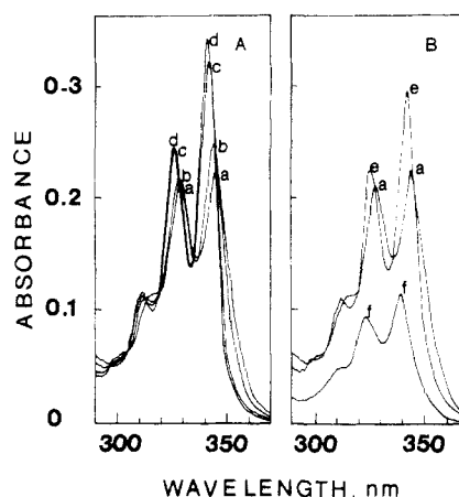
Figure 8. (A) Absorption spectra of 1 \times 10^{-5} M C 11 PN + in aqueous solutions of PMA at pH 8 on the addition of C 10 TAB, 10^{-3} M: (a) 0, (b) 2.0, (c) 3.0, (d) 8.0. (B) Absorption spectra of 1 \times 10^{-5} M C 11 PN + in aqueous solutions of PMA at pH 8 (a), pH 2 (e), and in water (f).
