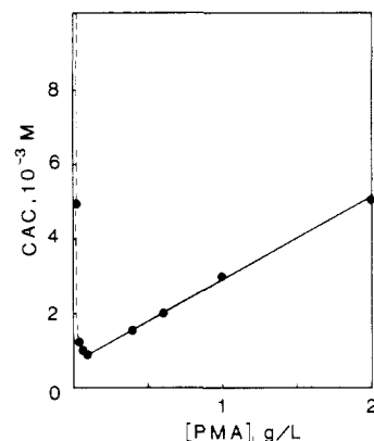
Figure 5. Dependence of the CAC of C_{10} TAB in aqueous solutions of PMA on the concentration of [PMA], g/L.
